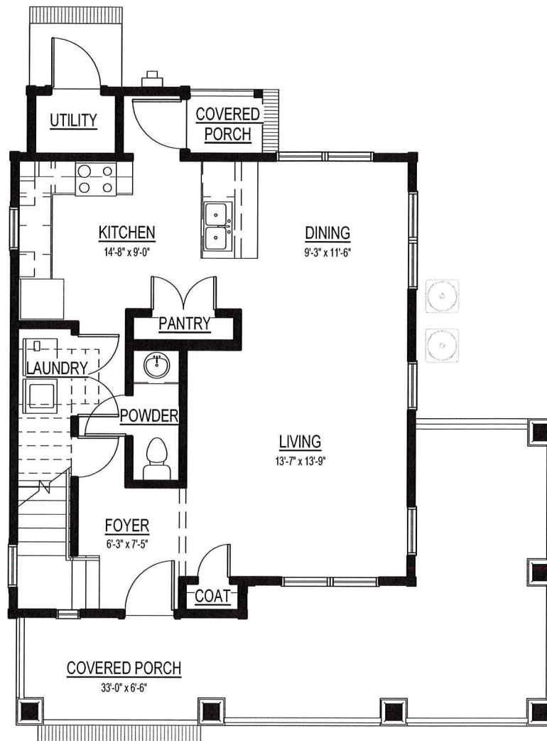
FIRST FLOOR OPTION B
