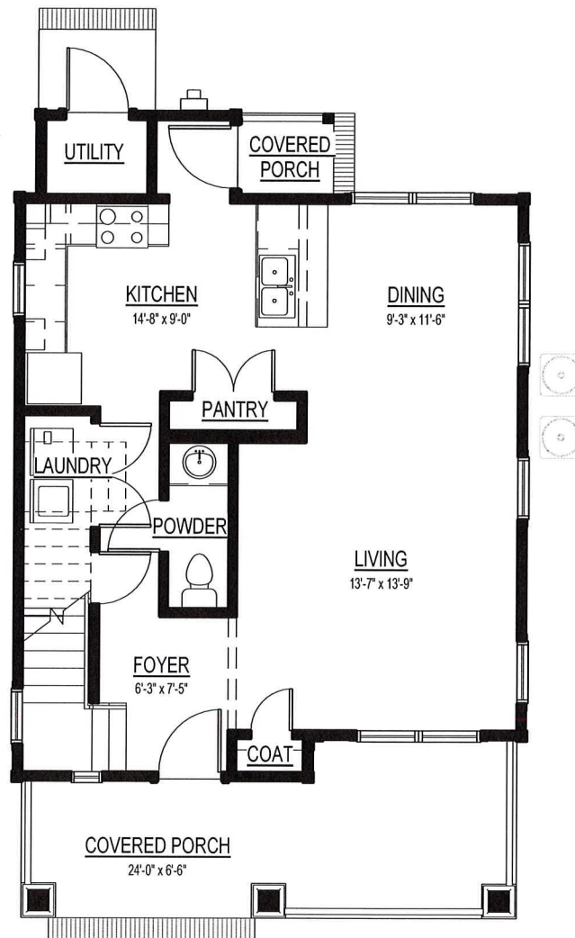
FIRST FLOOR OPTION A
